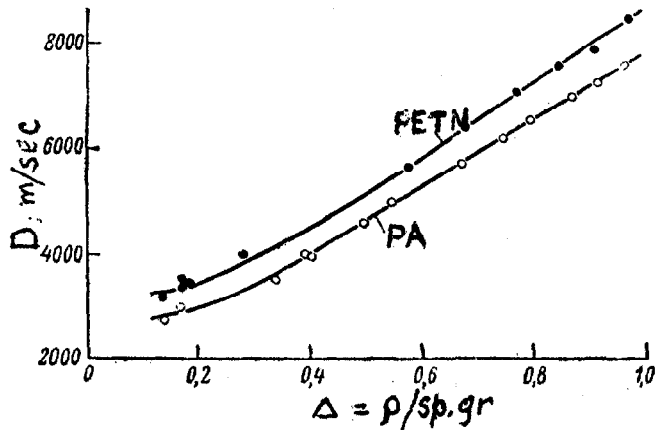
Fig 5 Relationship: Detonation Velocity (D) vs "Relative Density" A
